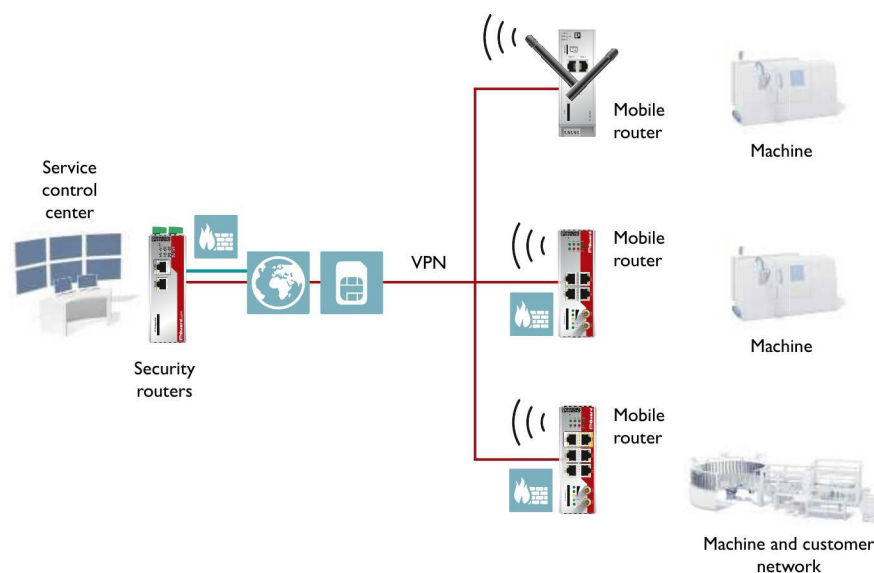
VPN communication via the mobile phone network
